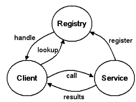
Figure 1. The Basic GridRPC Model.
